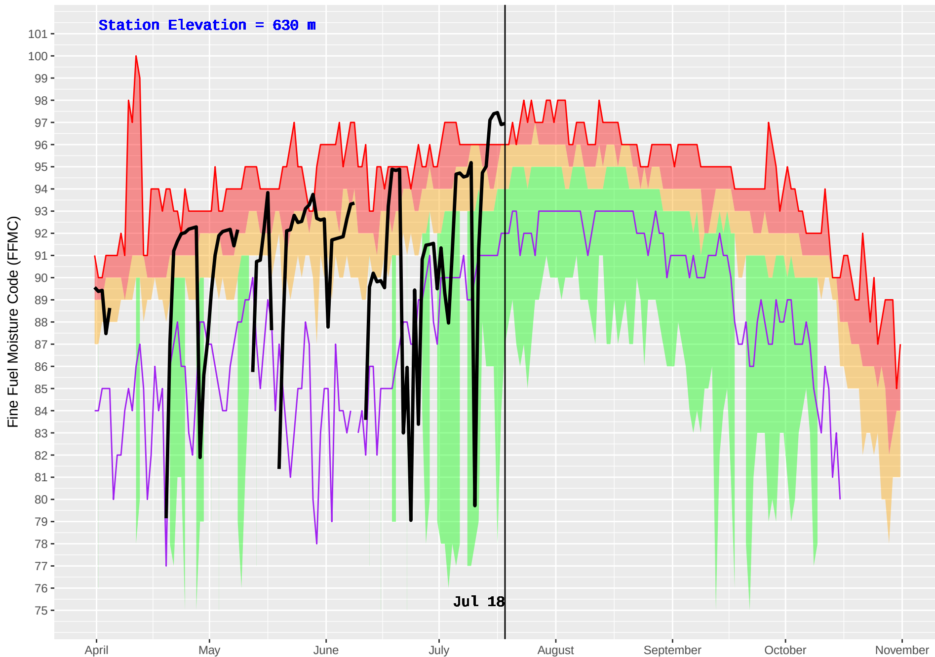
GRAND FORKS (392) : Historical (1981–2016) and Current (2018) Daily Fine Fuel Moisture Code (FFMC)
