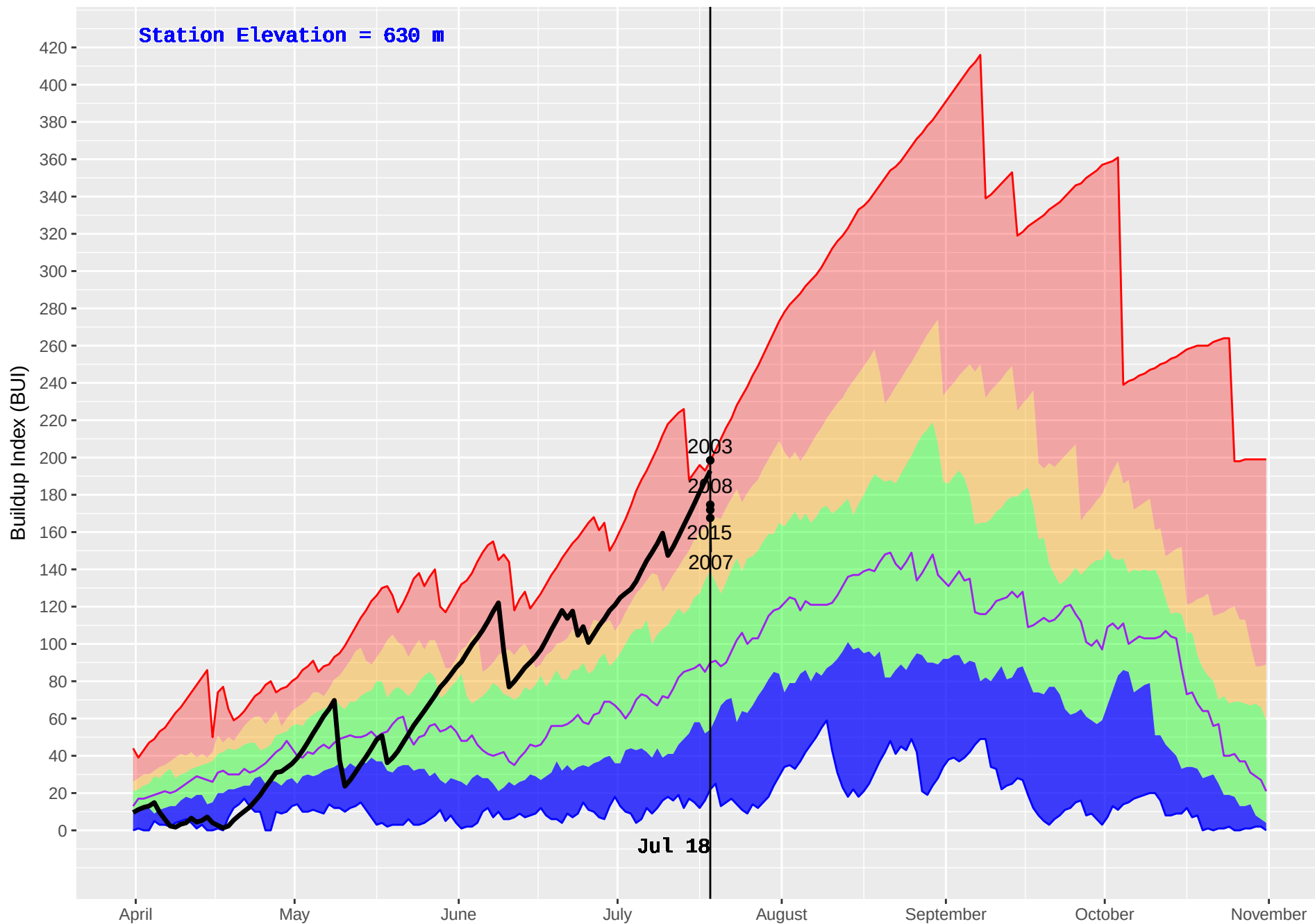
GRAND FORKS (392) : Historical (1981–2016) and Current (2018) Daily Buildup Index (BUI)
